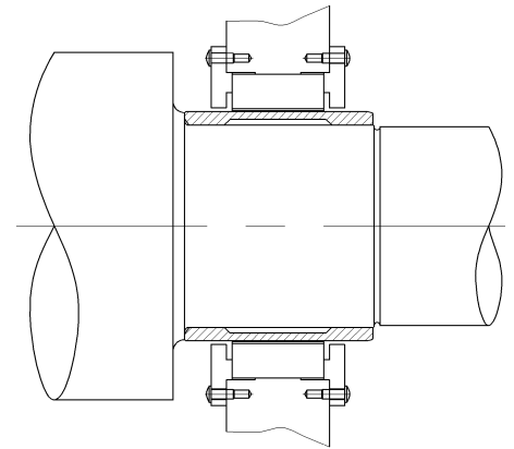
Figure 13. Typical Heat Barrier Sleeve (patent protected)
