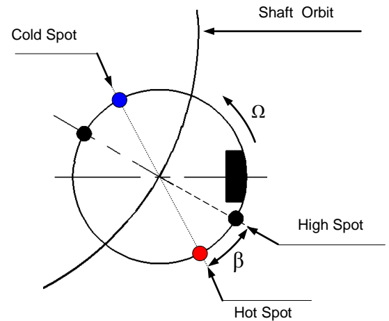
Figure 3. Journal Cross-Section Showing Phase Lag \beta between High Spot and Hot spot
