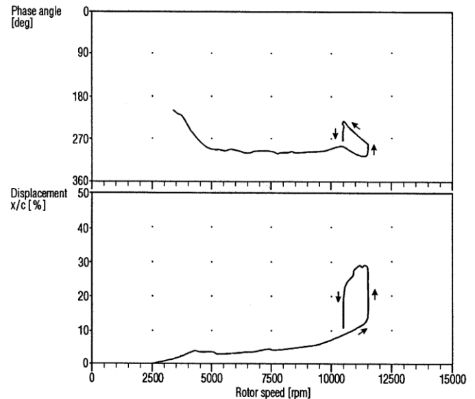
Figure 6. Bode Plot (1x) with Typical Hysteresis Loop (de Jongh and Morton, 1994)
