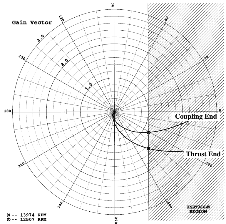
Figure 9. Complex Gain Vector for the Gas Boost Compressor (Kocur and de Jongh, 2000)
