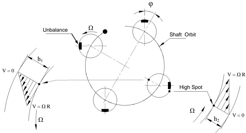
Figure 2. Differential Heating at Bearing Journal for Synchronous Forward Rotor Whirl
