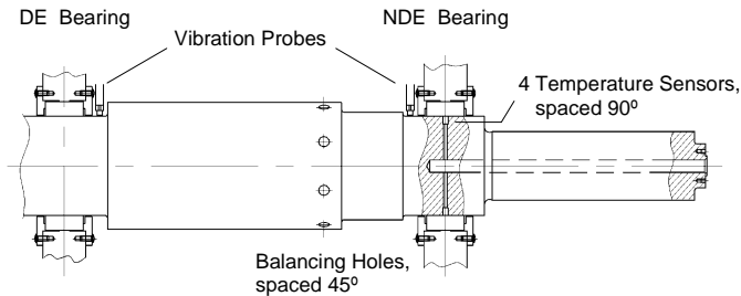
Figure A-1. Test Rotor with Four Temperature Sensors at the NDE Bearing.
