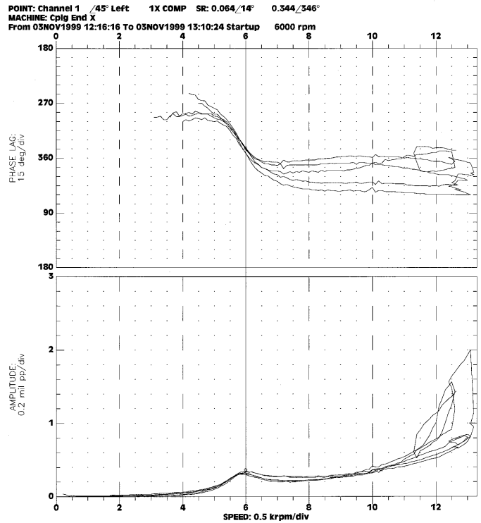
Figure 10. Synchronous Vibration on Test Stand (Coupling End) (Kocur and de Jongh, 2000)
