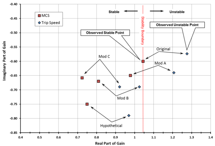
Figure 11. Predicted Thermal Gain of Various Coupling Configurations (Kocur and de Jongh, 2000)
