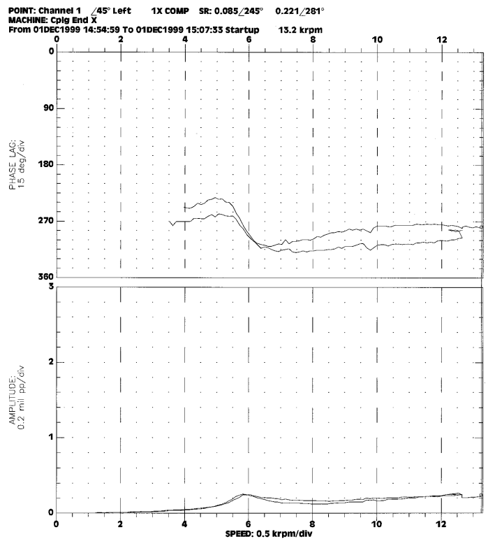
Figure 12. Synchronous Vibration with Reduced Coupling Overhung Moment (Kocur and de Jongh, 2000)
