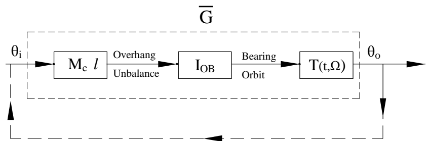
Figure 5. Scheme of Synchronous Instability Phenomenon
