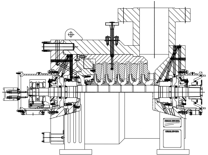
Figure 8. Cross-Section of 30,000 HP Gas Boost Compressor (Kocur and de Jongh, 2000)
