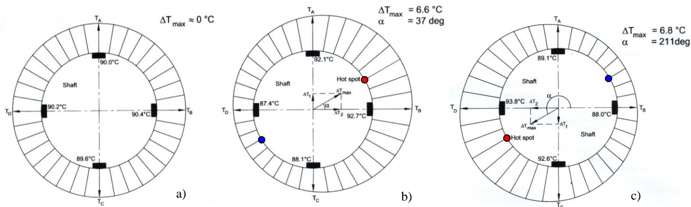
Figure A-3. Cross-Section of NDE Bearing Journal, with Sinusoidal Temperature Distribution.
